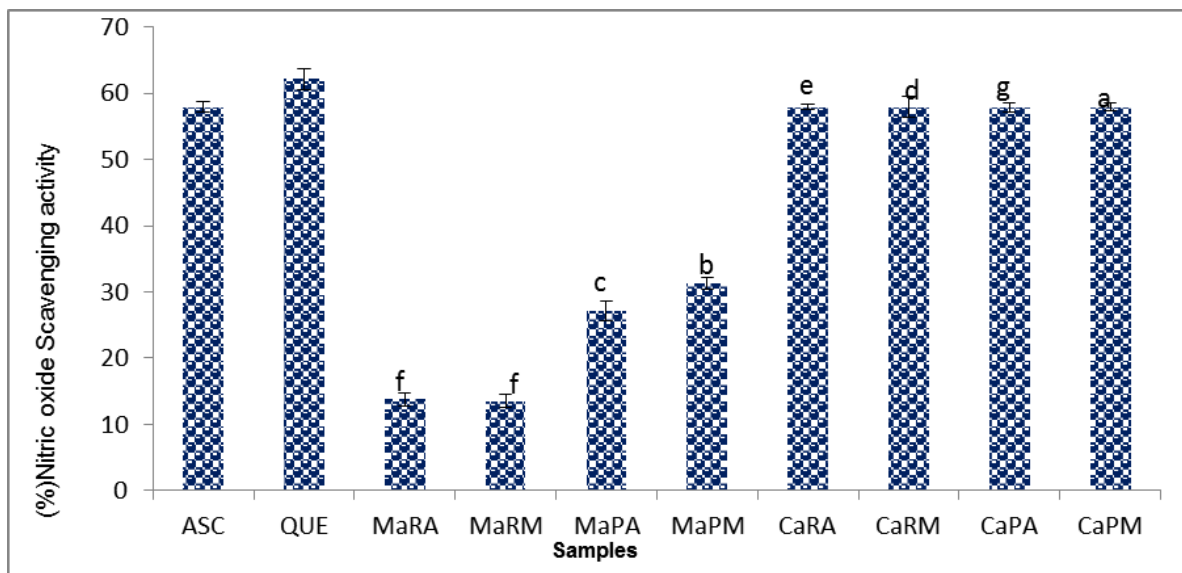
Fig 1: Nitric oxide radical scavenging activity of aqueous Acetone and Methanol extract of M. arudinaceae and C.amada rhizomes.
